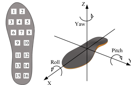
Fig. 3. The position of a 16 pressure sensors array in the insole (left). Roll, pitch, and yaw angles can be described as rotational angles around x-, y-, and z-axes of the insole in a world frame (right).
