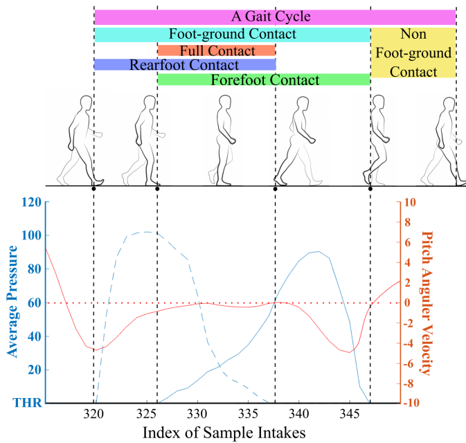
Fig. 4. Blue solid/dashed graph: The forefoot/rearfoot average pressure trend of a healthy subject extracted by SITUG during a gait cycle. Red solid graph: The pitch angular velocity of the subject in the gait cycle. Spatial-temporal features including forefoot contact, rearfoot contact, full contact, foot-ground contact, and foot-ground non-contact times are marked regarding the average pressure trends. All these features and their relationships with the average pressures are described in Table II
